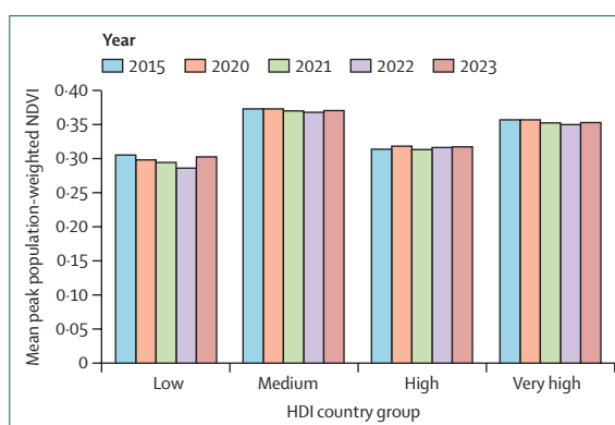
Figure 5: Mean population-weighted peak-season NDVI of urban centres by HDI and year NDVI=normalised difference vegetation index. HDI=Human Development Index.
